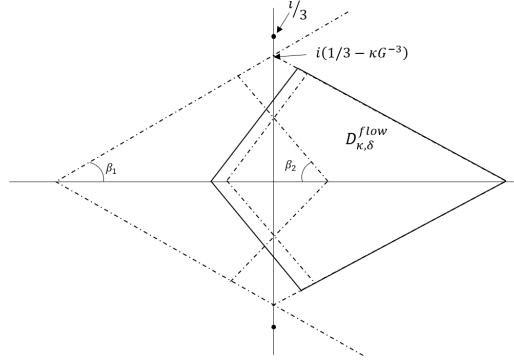
FIGURE 4.2. The domain D_{\kappa, \delta}^{\text{flow}} defined in (4.4).
